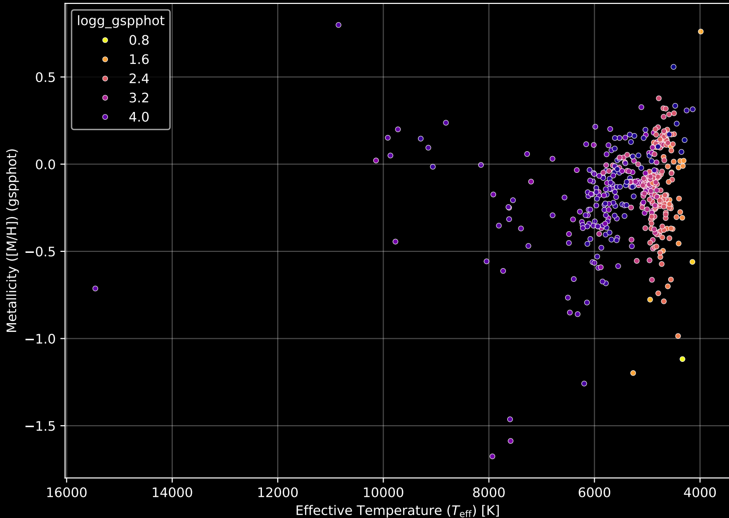
APOGEE DR17 Field: [K01_082+17] Stellar Population Parameters (n= 419)
