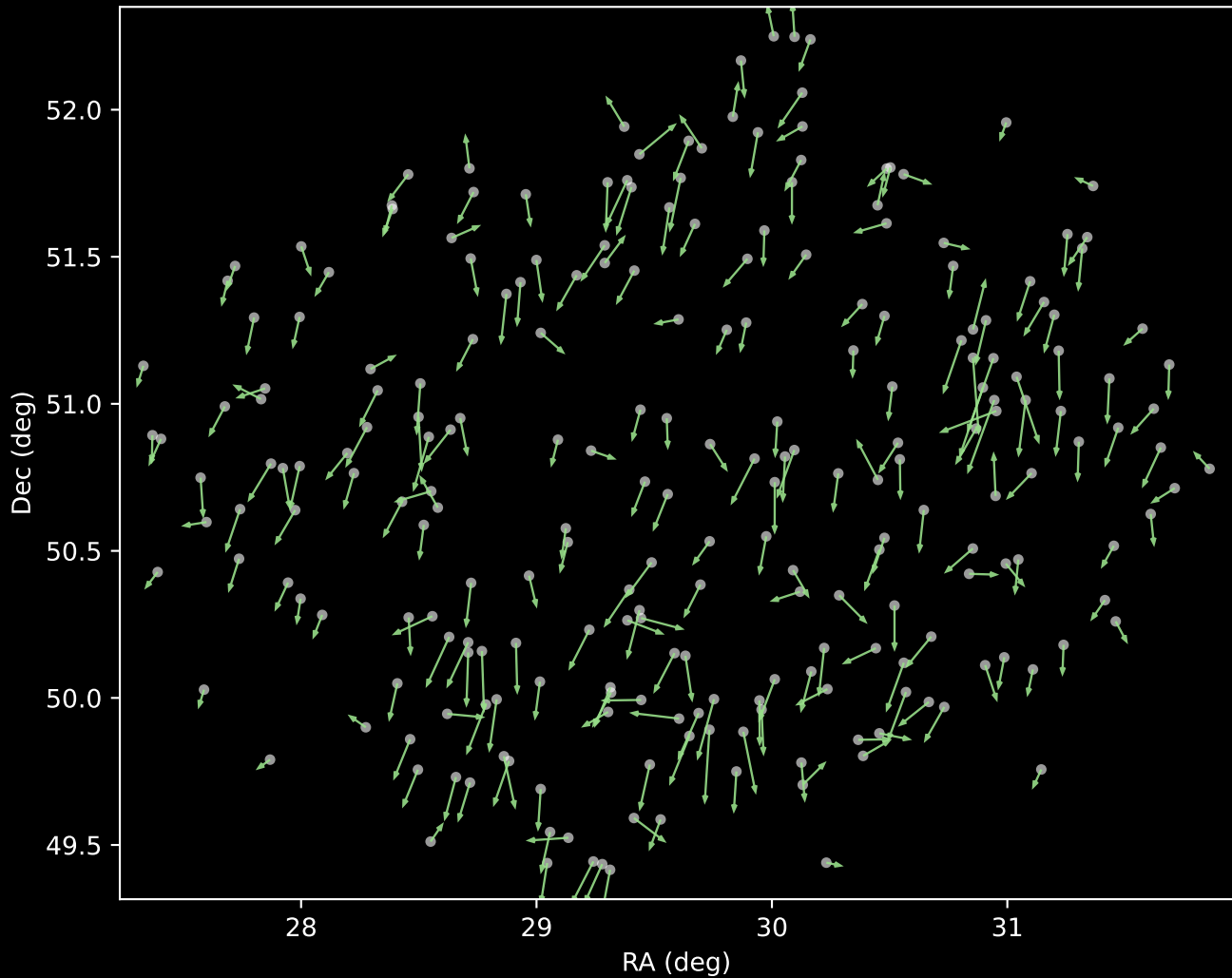
APOGEE DR17 Cluster 5 Proper Motion Vectors (n=236)
