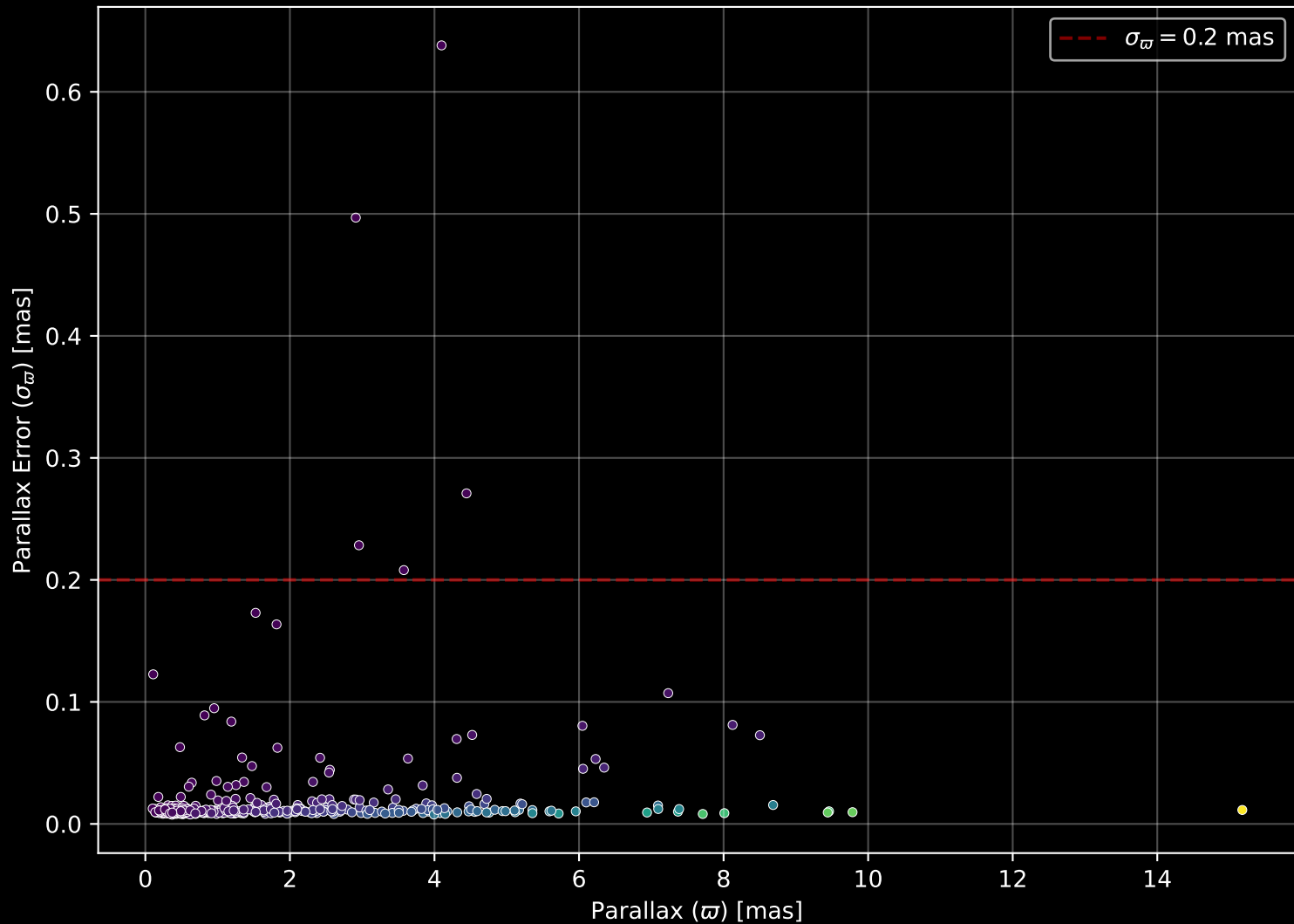
APOGEE DR17 Field: [K01_082+17] Parallax Quality (n= 419)
