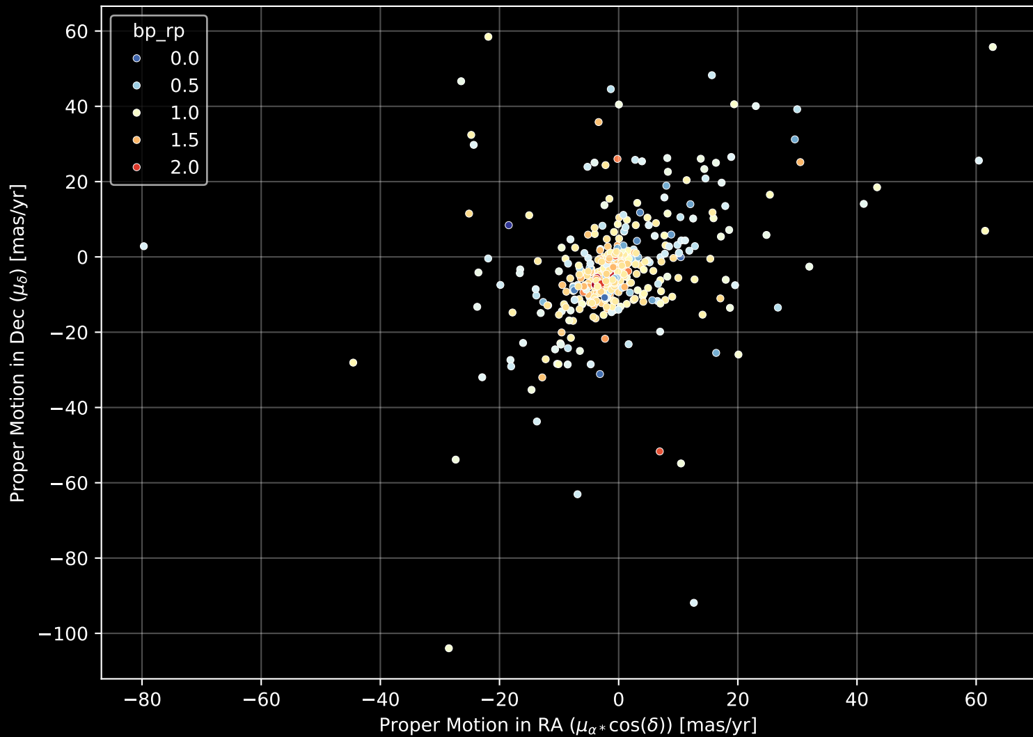
APOGEE DR17 Field: [K01_082+17] Proper Motion Diagram (n= 419)
