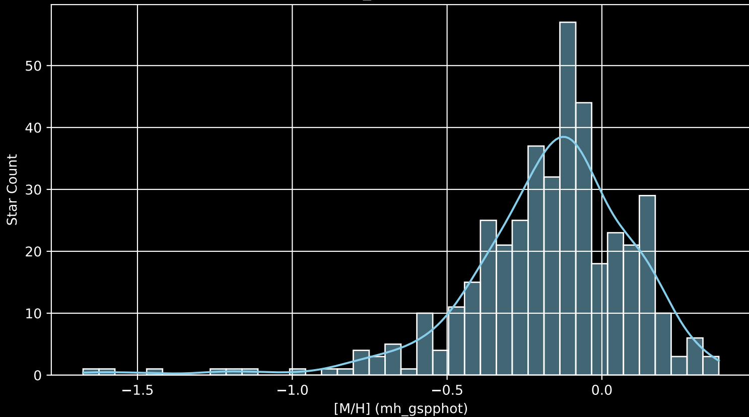
APOGEE DR17 Field: [K01_082+17 [M/H] (mh_gspphot) (n= 416)
