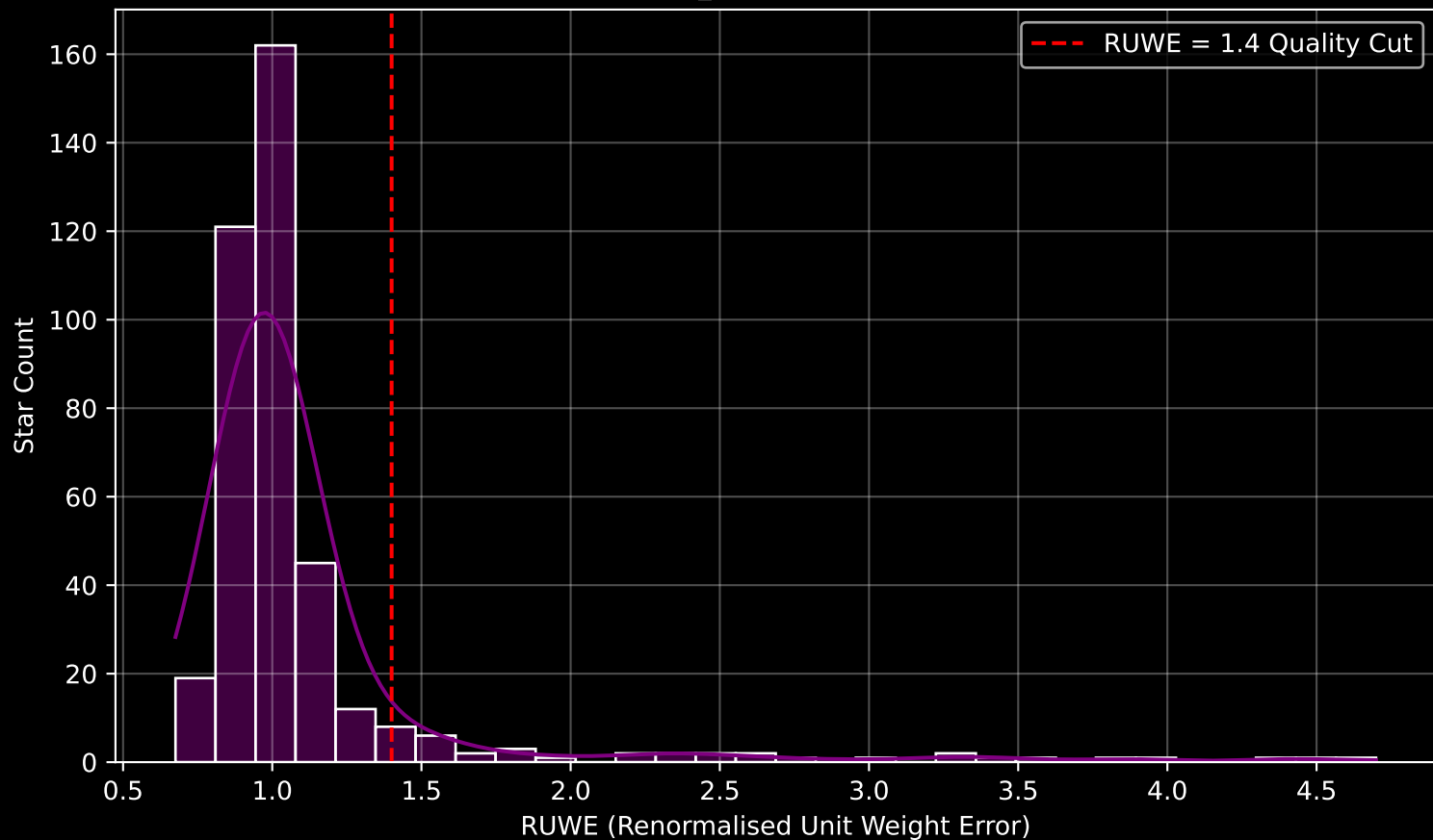
GAPOGEE DR17 Field [K01_082+17] RUWE Distribution (n= 398)
