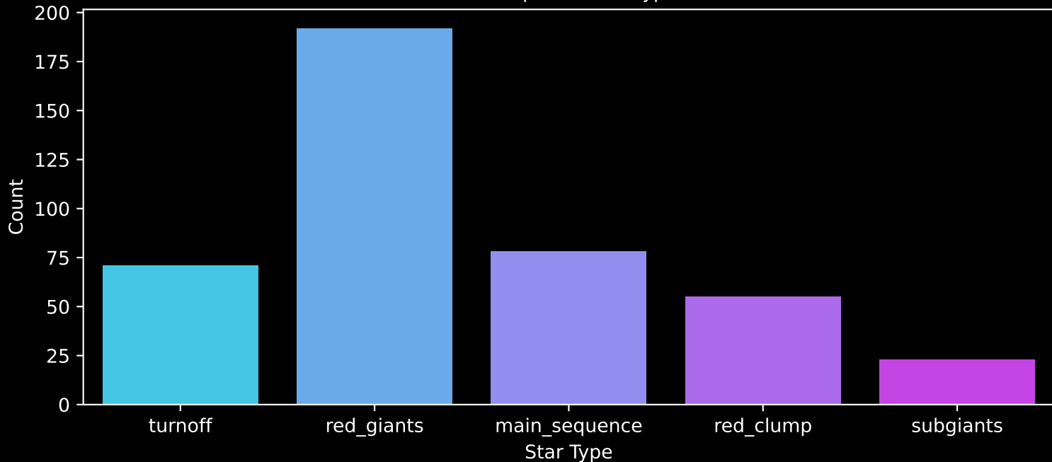
APOGEE DR17 Field: [K01_082+17] Count plot of Star Type
